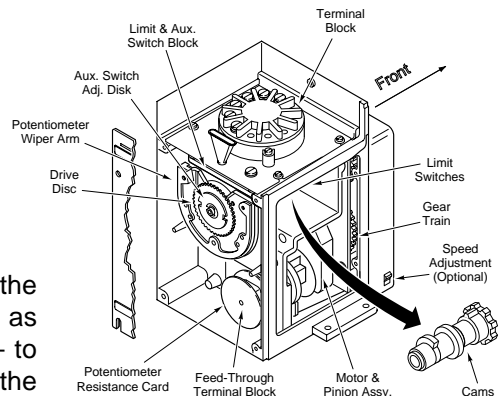
Figure 8. Exploded View
